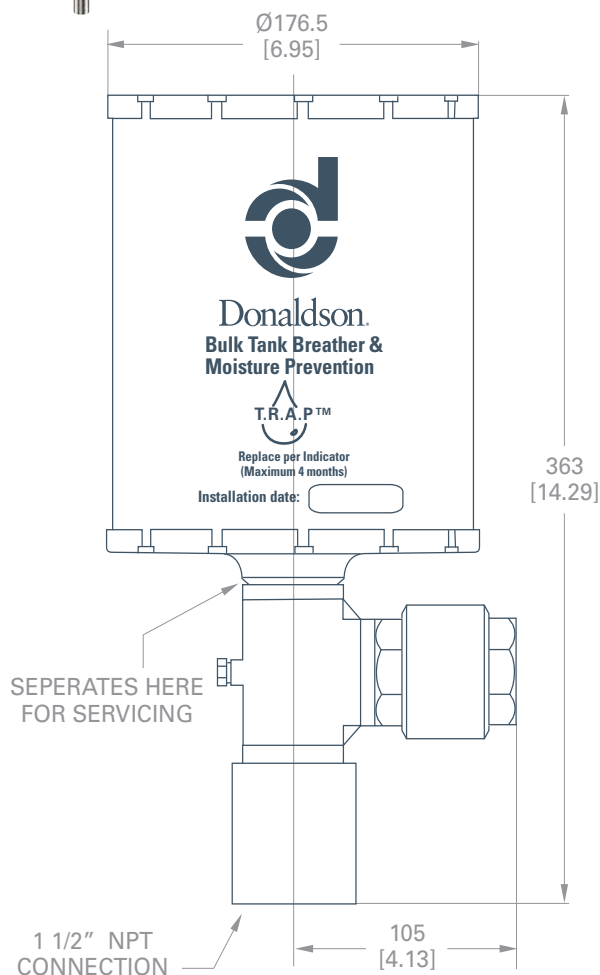
T.R.A.P. Breather X920006
