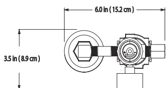
Reservoir Air Vent P575852
