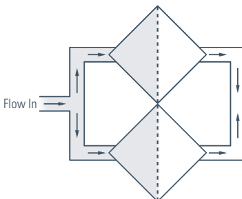
Dual Head With Parallel Flow Path
