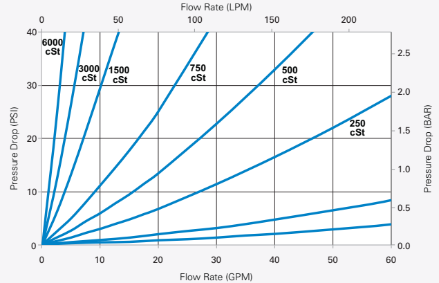
DBB8664 - Heavy Oil Filter
