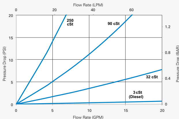
DBB7733 - Compact Winter Fuel Filter
