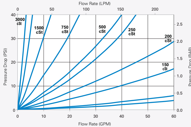
DBB8665 - Light Oil Filter
